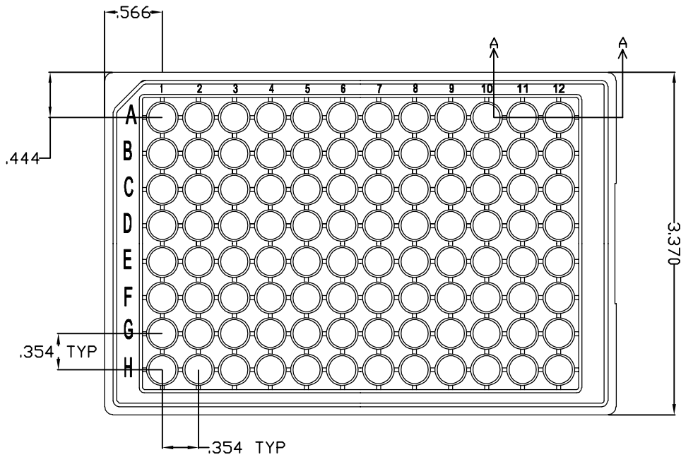
TOP VIEW SHOWN WITHOUT COVER
